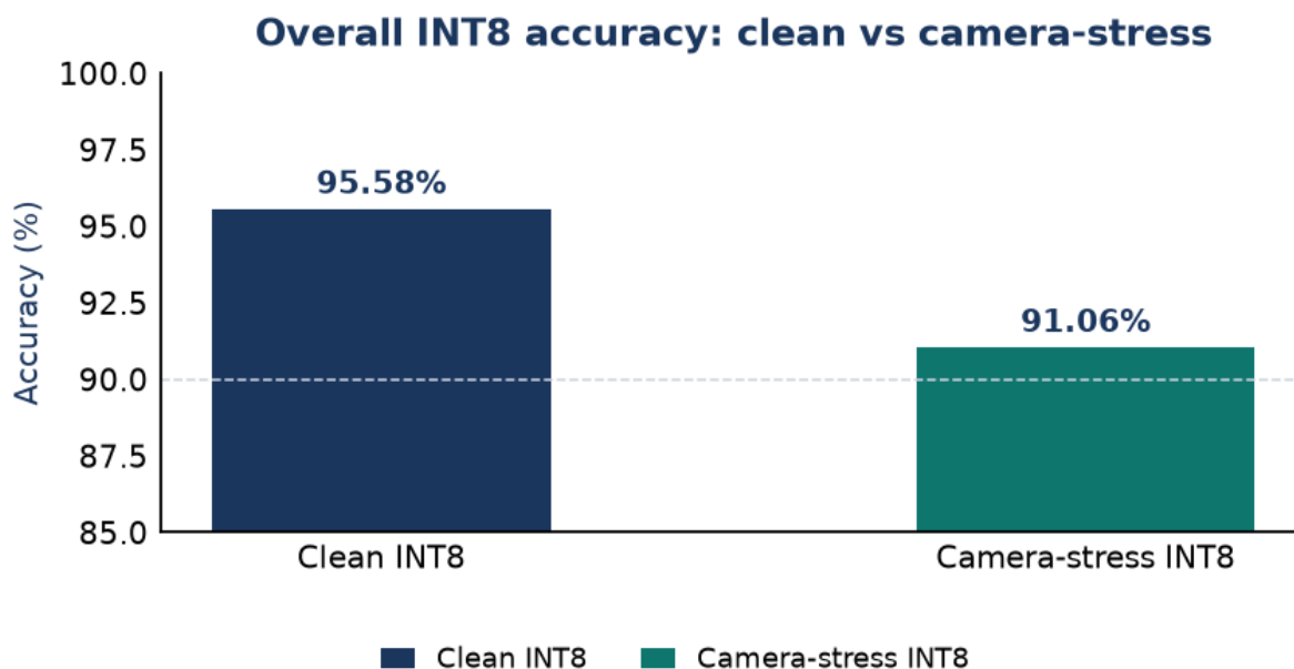
Figure 1. Overall INT8 accuracy on the same test set (n = 4,319). Camera-stress applies blur + JPEG + underexposure. Dashed line is the 90% notebook target.
