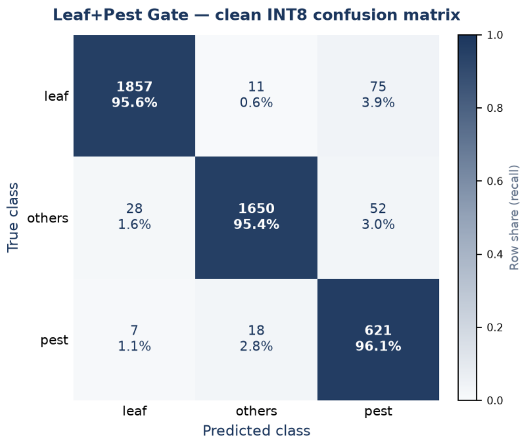
Figure 3. Leaf+Pest Gate confusion matrix, clean INT8 test ( n = 4,319 ).
