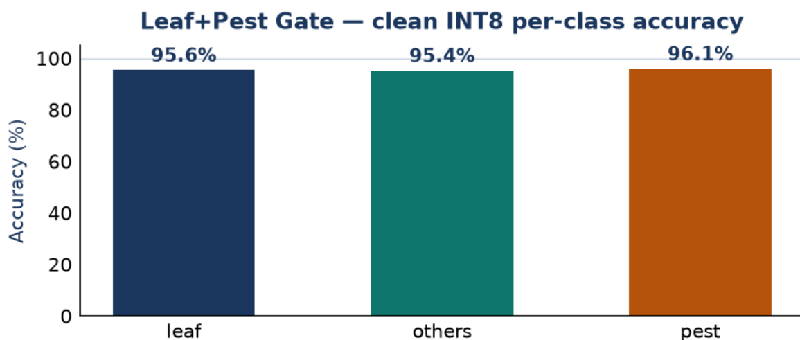
Figure 2. Clean INT8 per-class recall. Pest is the smallest class but the most accurate.
